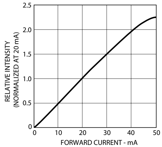
Figure 4: Relative Intensity vs Forward Current
